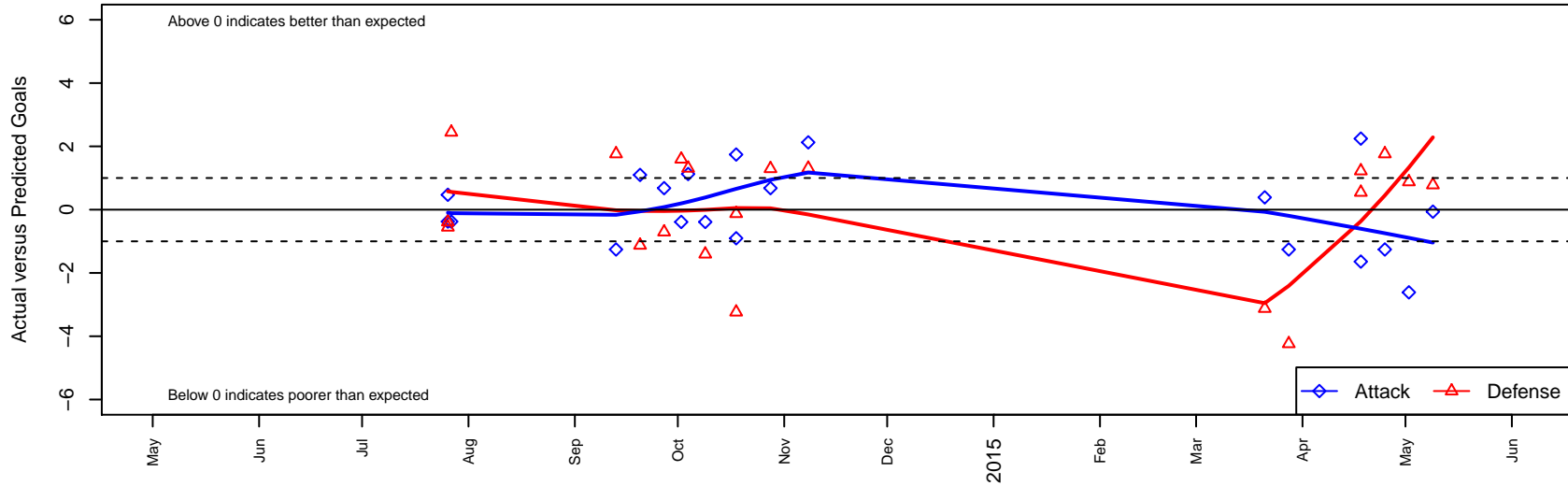
ASE Navy G03 Dots are actual minus expected GF (blue circles) and GA (red triangles). Blue line is smoothed change in attack strength. Red is smoothed change in defense strength.
